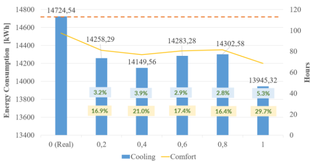
Figure 5. Variation of the depth of the overhang.
