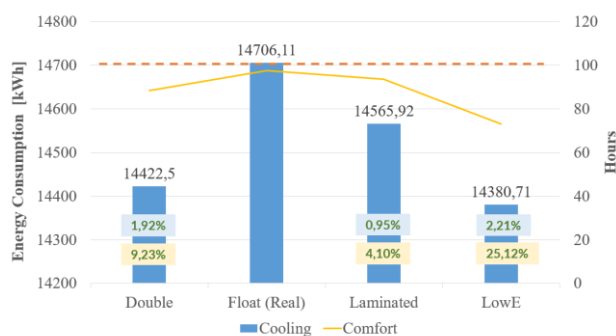
Figure 6. Variation in glass type.
