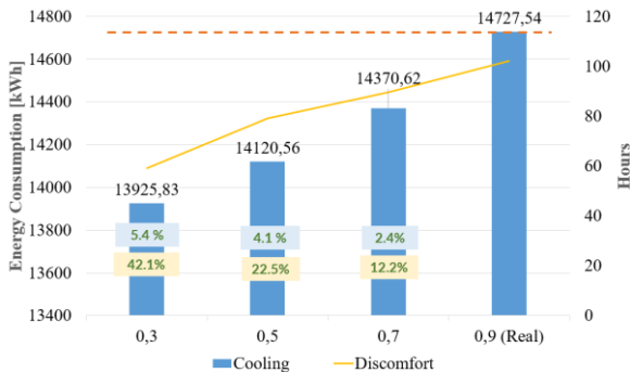
Figure 4. Variation of the solar absorbance of the roof.
