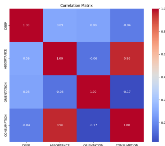
Figure 8. Correlation analysis of parameters with cooling energy consumption.
