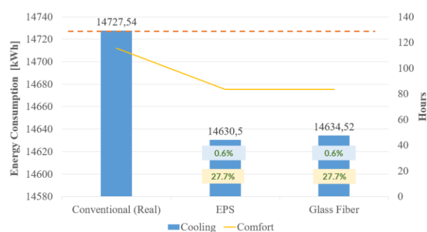
Figure 7. Variation of the type of Wall.
