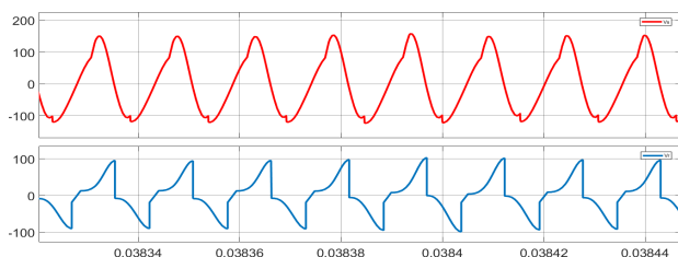
Figure 9. Vs & Vr waveforms for WPTS with Class-E inverter and d=10cm.
