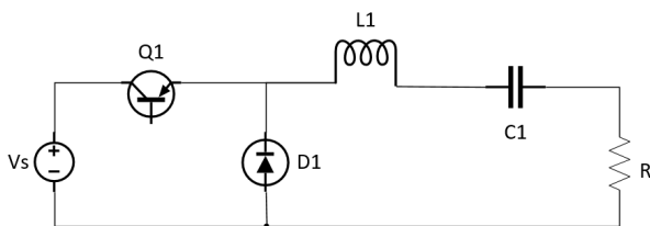
Figure 4. Buck converter basic circuit diagram.
