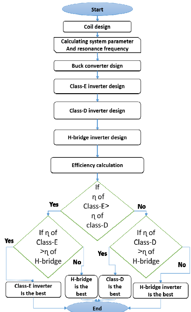
Figure 8. Flow chart depicting the process of designing WPT and a comparison of inverters.
